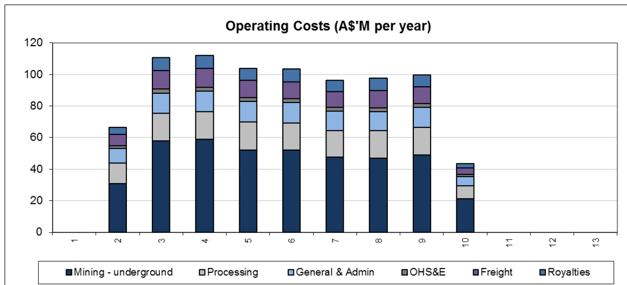
Figure 8 - Savannah FS Optimisation - Annual operating costs
