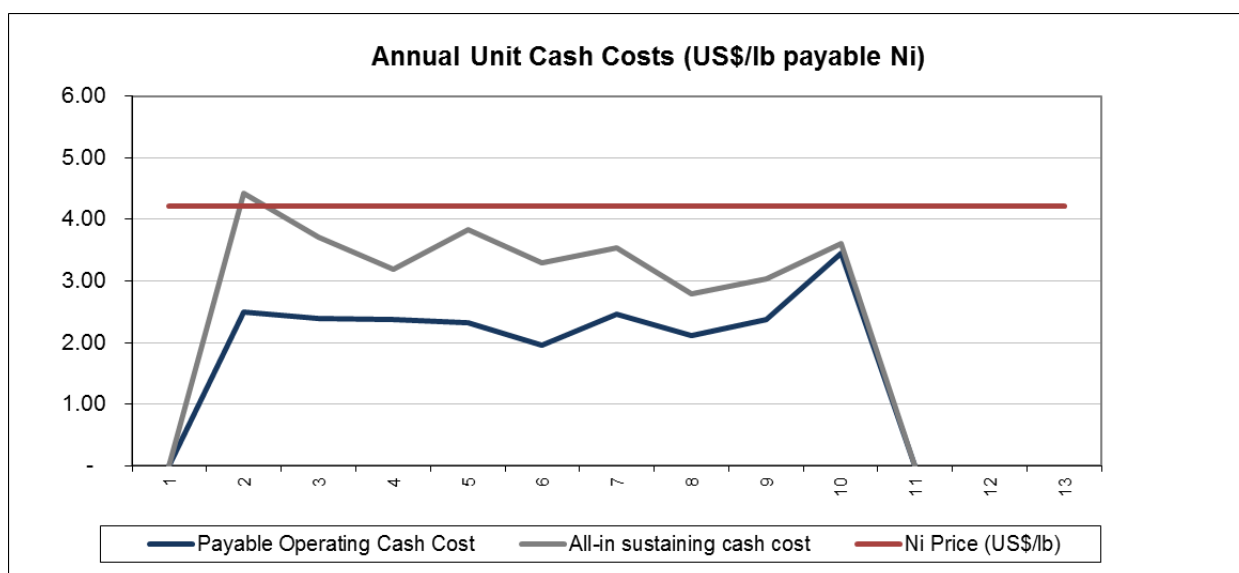
Figure 9 - Annual unit operating and sustaining cash costs (US$ per pound payable nickel)
