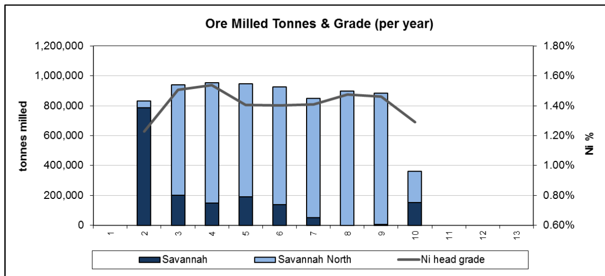
Figure 4 - Savannah Optimisation – Annual production and grade profile
