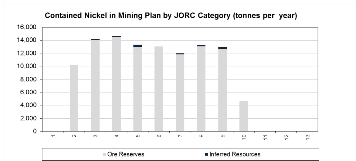
Figure 2 - Savannah Optimisation – Annual nickel in material mined by JORC category
