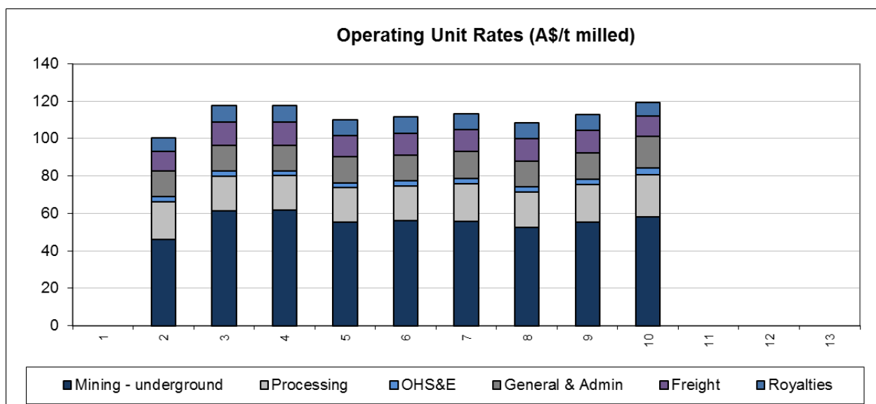
Figure 7 - Savannah FS Optimisation - Annual unit operating costs per tonne milled
