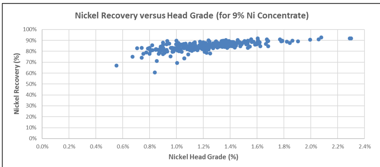
Figure 3 - Historical Savannah plant nickel recovery versus head grade for a concentrate grade of 9% Ni
