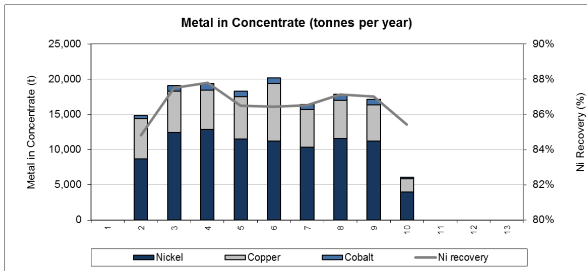
Figure 5 - Annual nickel processing recovery and metal in concentrate production
